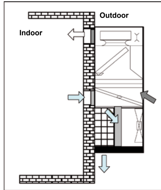
Fig.3 - FREE COOLING
