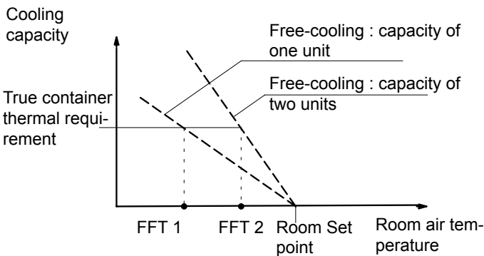
Fig.6 - SFT® operating diagram
