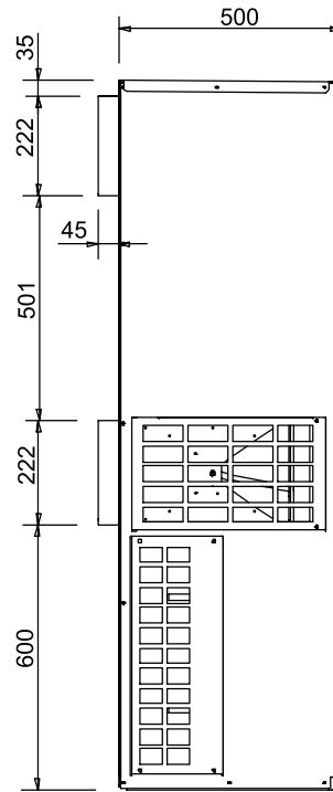
Side view
