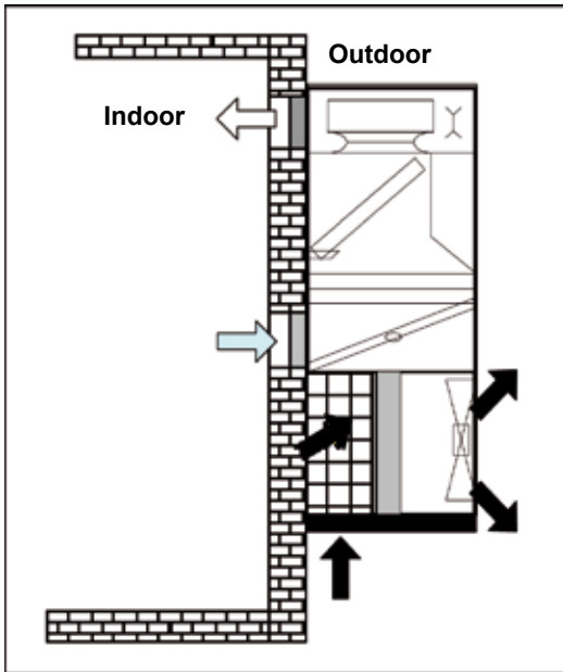
Fig.2 - MECHANICAL COOLING
