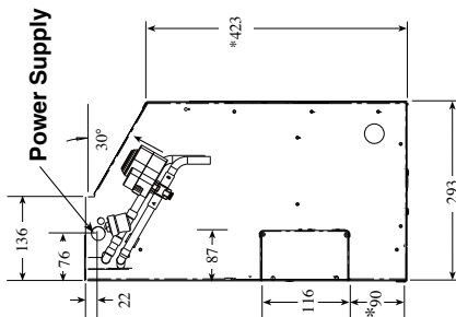
Left Hand Configuration (Bottom Return)
